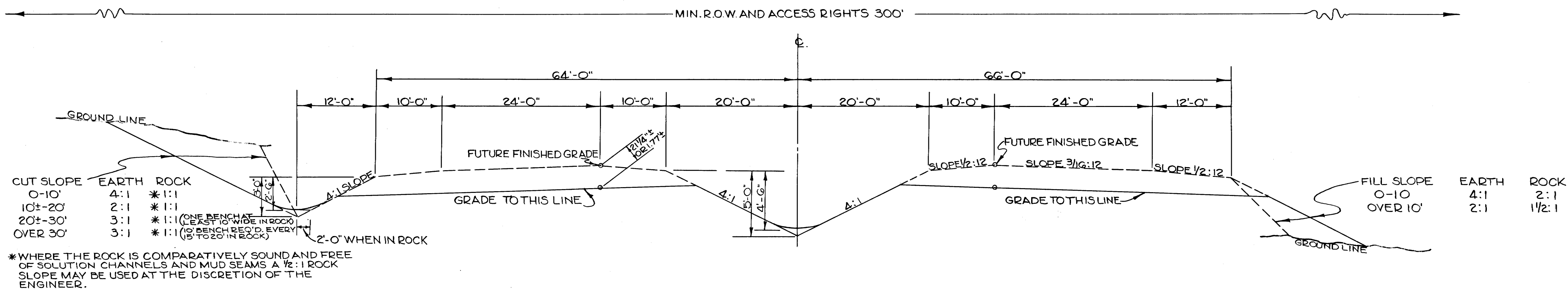
TYPICAL SECTION NO. 1 TYPICAL CROSS-SECTION OF INTERSTATE WITH 60' MEDIAN (TANGENT SECTION)
