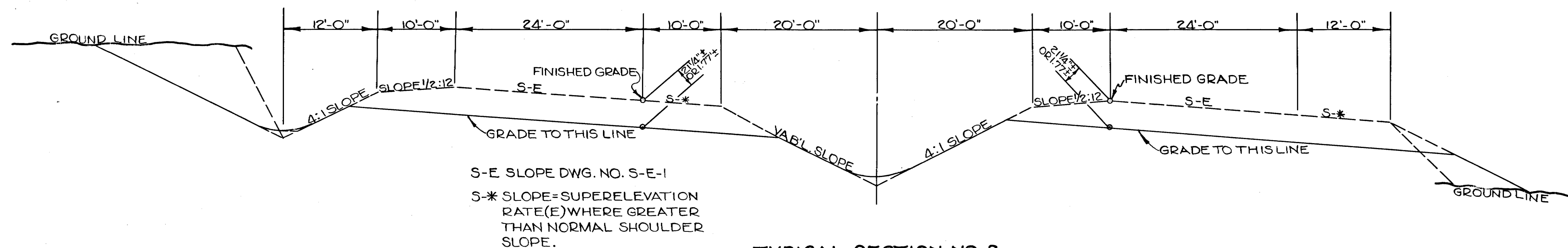
TYPICAL SECTION NO. 2 TYPICAL CROSS-SECTION OF INTERSTATE (ON SUPER-ELEVATED SECTIONS-DETAILS NOT SHOWN SAME AS T
